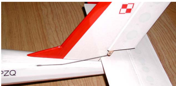
17. Insert rudder pushrod to the horn and then glue hinges with small amount of thin CA.
