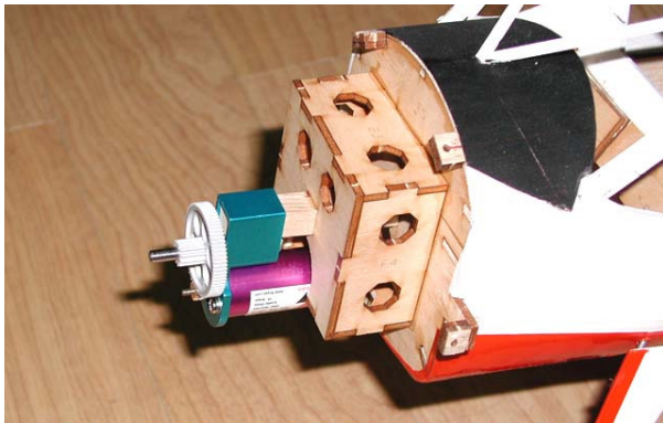
15. Install motor and gearbox.
