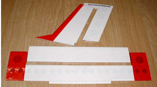
5. Make hinge slots and pre-install hinges. (Do not glue hinges in this step.)
