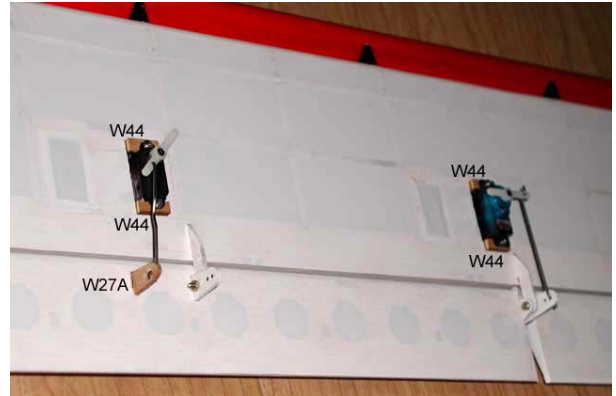
10. If required, glue optional plywood servo beds(W44). You may use a servo reverser when you connect flap servos with Y-harness, if not, install optional flap horn(W27A).
