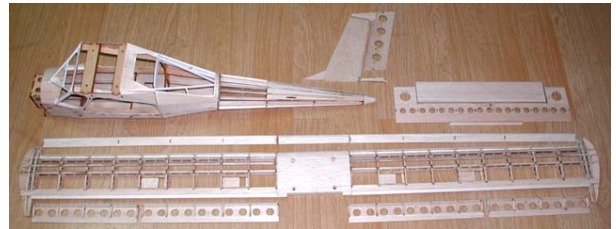
23. All the airframes are ready to cover.
