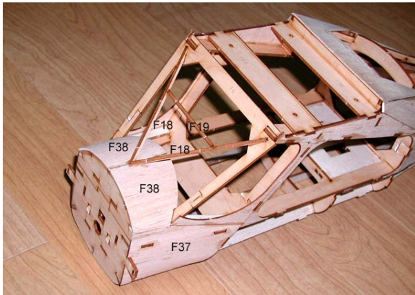
15. Glue fore cockpit frames(F18, F19), turtle decks(F38) and fore side panels(F37).
