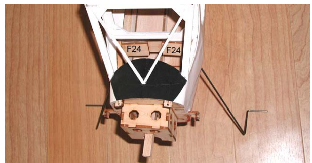
13. Glue landing gear retainer(F24).
