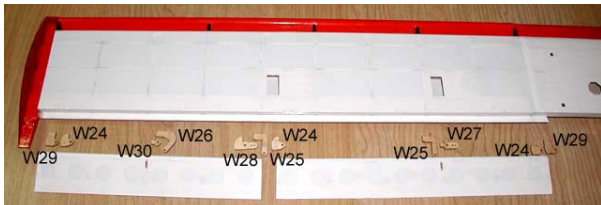
7. Prepare aileron and flap hinges and horns(W24-W30).
