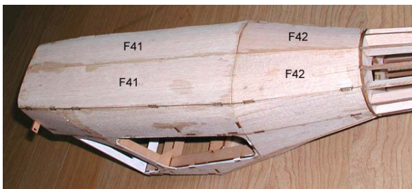
18. Glue fuselage lower panels(F41, F42).
