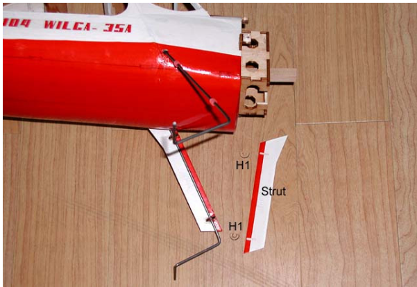
14. Assemble dummy landing gear with silicon tubes, holders(H1) and landing gear struts.
