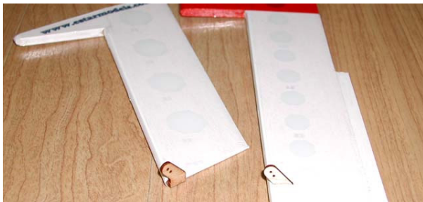
16. Install and glue elevator and rudder plywood horns. Apply thin CA to the horns for reinforcing.
