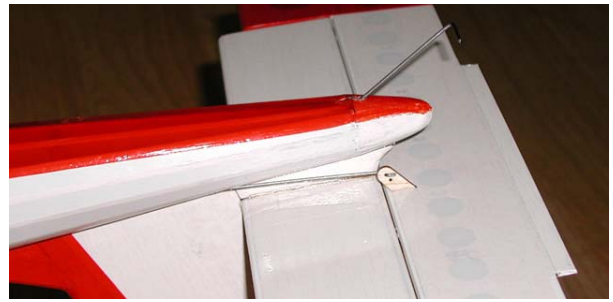
18. Insert elevator pushrod to the horn and then glue hinges with small amount of thin CA.
