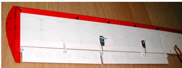
9. Install aileron and flap servos and connect pushrods.
