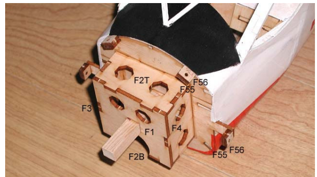
11. Assemble plywood motor mount box(F2-F4) and cowl mounts(F55, F56). Make sure to pay attention to bulkhead F1 the numbers should be facing forward.
